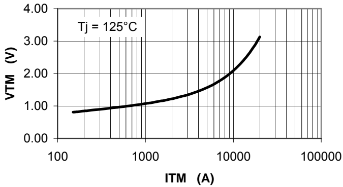
Maximum On-State Voltage Drop
