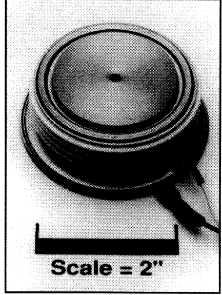
T9K7 800A Phase Control SCR 800 Amperes Average, 4500 Volts
