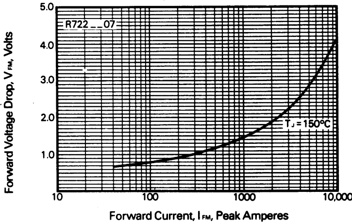
Forward Voltage Drop vs. Forward Current
