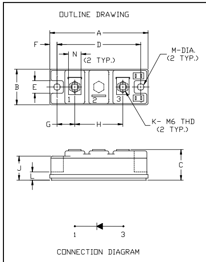
QRS0660T30 Fast Recovery Diode Module
