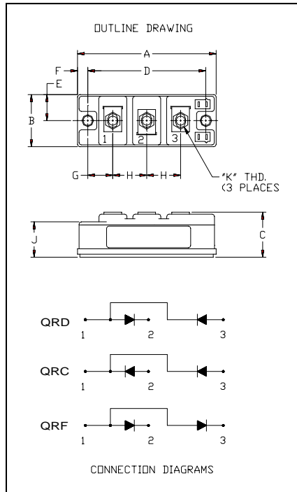
QR_1415T30 Fast Recovery Diode Module
