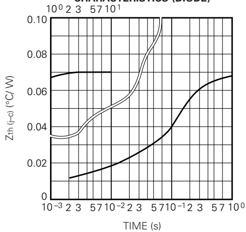
TRANSIENT THERMAL IMPEDANCE CHARACTERISTICS (DIODE)
