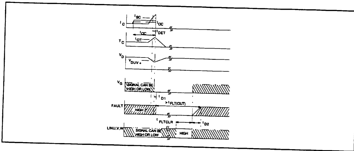
Fig. 10 - Timing Diagram
