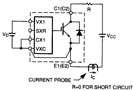
Figure 5 Over Current and Short Circuit Test
