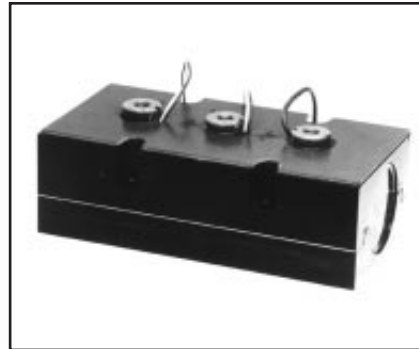
POW-R-BRIK™ Phase Control Modules 345-800 Amperes/400-3000 Volts
