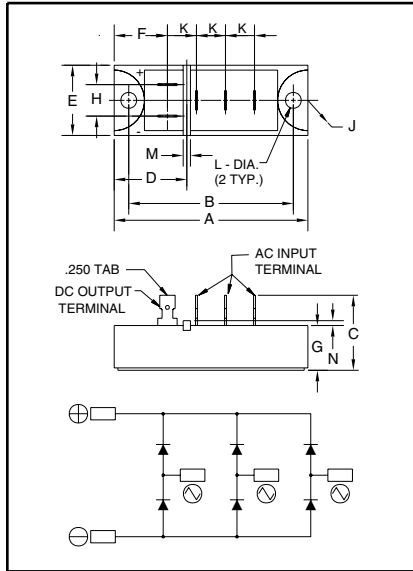
ME700802 Three-Phase Diode Bridge Modules 20 Amperes/800 Volts
