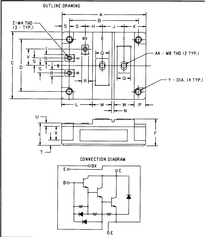
Outline Drawing
