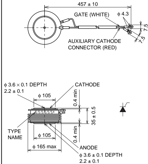
OUTLINE DRAWING
