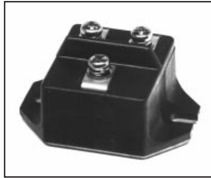
CN24__020N, CC24__020N Super Fast Recovery Dual Diode Modules 20 Amperes/300-600 Volts
