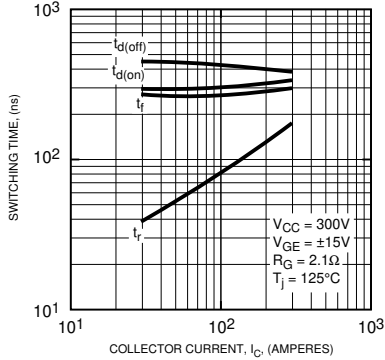
HALF-BRIDGE SWITCHING CHARACTERISTICS (TYPICAL)
