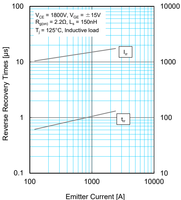
FREE-WHEEL DIODE REVERSE RECOVERY CHARACTERISTICS (TYPICAL)
