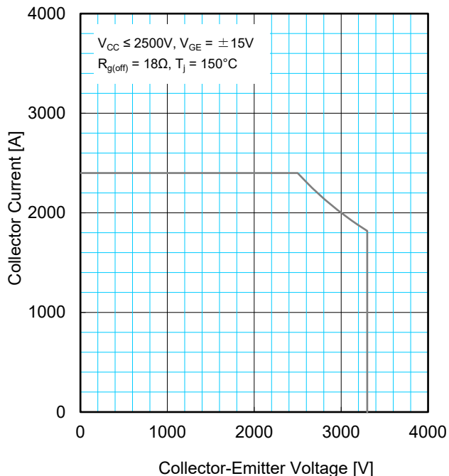
REVERSE BIAS SAFE OPERATING AREA (RBSOA)
