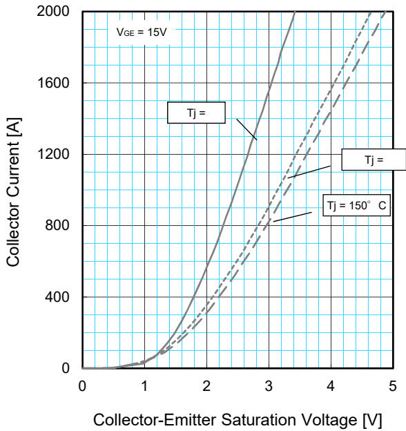
COLLECTOR-EMITTER SATURATION VOLTAGE CHARACTERISTICS (TYPICAL)
