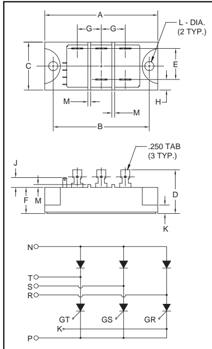
Outline Drawing
