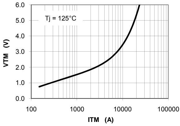
Maximum On-State Voltage Drop
